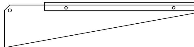
Rakks T-Style Lab Bracket
