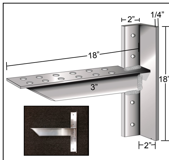
EHB INSIDE WALL Bench Bracket
